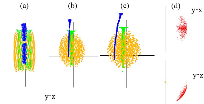
Figure 4: (Color) The time sequence of 1 \times 10^{22} \text{W/cm}^2 (Run A4) for enlarged yz plots at (a) 3fs, (b) 10fs, (c) 21fs, and (d) for reduced yx and yz plots, mainly of electrons, at 21fs. Protons are shown in blue, carbons by green, golds by gold, and electrons in red. The scales are 3.5 \times 10^{-6} \text{cm} , 1.2 \times 10^{-5} \text{cm} and 2.6 \times 10^{-5} \text{cm} in (a) to (c), respectively, and 6.2 \times 10^{-4} \text{cm} in two vertical plots (d).
