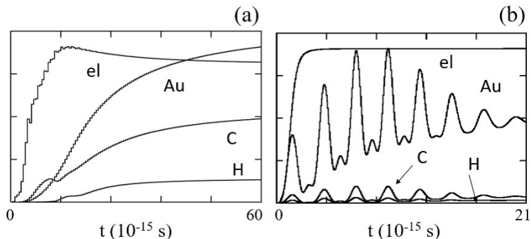
Figure 6: The time changes of kinetic energy of golds, carbons, protons, and electrons for (a) 5 \times 10^{17} \text{W/cm}^2 , and (b) 1 \times 10^{22} \text{W/cm}^2 . The maximum values are, (a) 0.59 MeV for ions (C,Au,H), and 0.33 MeV for electrons, (b) 42 MeV for golds, and 37 MeV for electrons, respectively. The final value of gold ions is 22 MeV for (b).
