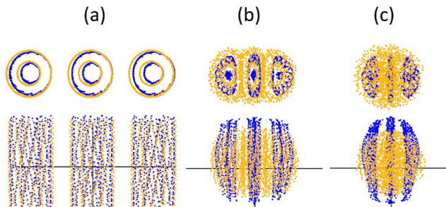
Figure 9: (Color) Merging of a three-array nanotube with double layers inside for (a) 1 fs, (b) 7 fs, and (c) 24 fs, and in carbon (blue) and gold (gold) ions. The scales in the yx (top) and yz (bottom) directions are, 1.3 \times 10^{-6} cm, 6.3 \times 10^{-6} cm, 2.5 \times 10^{-5} cm for (a) to (c), respectively.
